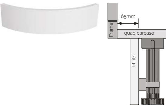
Quadrant pure curve plinth application Ref: PREFIX-CURVEPLINTHSCD
