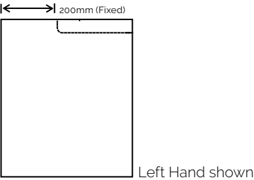
Horizontal Extended Stop Profile
