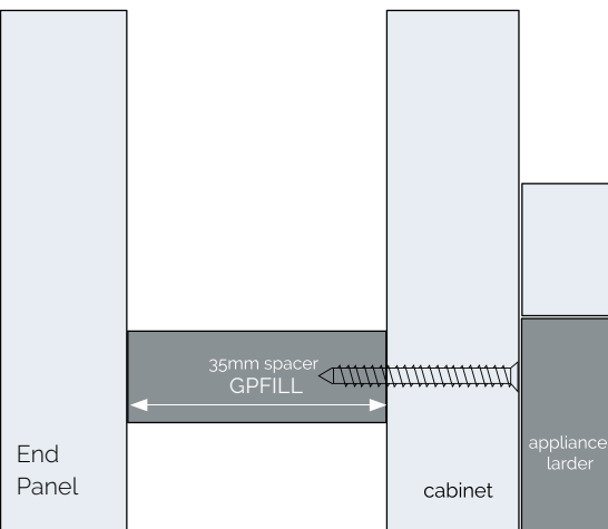
Spacer detail (back of unit)
