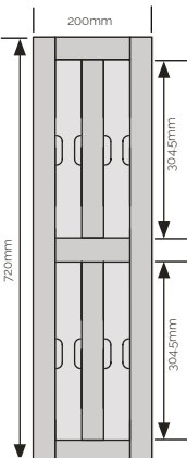
Chopping board set Ref: PREFIX-720200CHOPSET4
