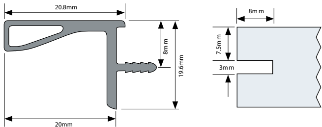
Rail profile
