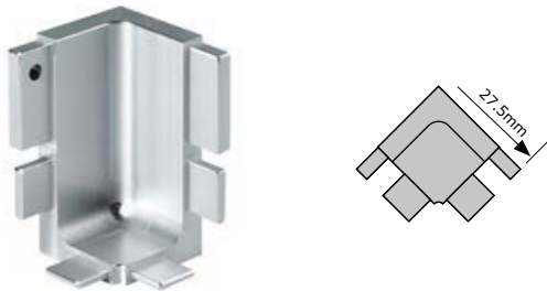
Fitted detail
