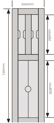
Tray set & chopping boards Ref: PREFIX-720200CHPTRYSET
