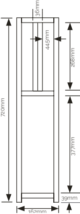
Carcase Assembly Using 18mm MFC Veneered Panels
