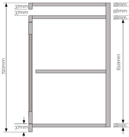
How to build your chopping board carcase
