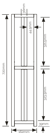
Carcase Assembly Using 18mm MFC Veneered Panels
