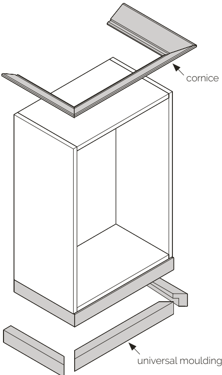
Cornice and pelmet application
