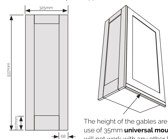
Wall framed end panel 937mm
