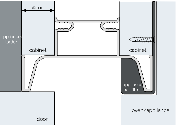
Appliance rail filler detail
