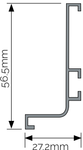
Rail profile
