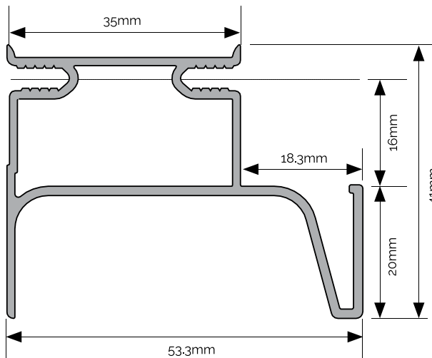
Rail profile
