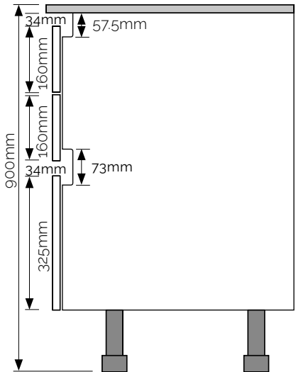
Cabinet dimensions
