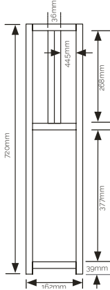
Carcase Assembly Using 18mm MFC Veneered Panels
