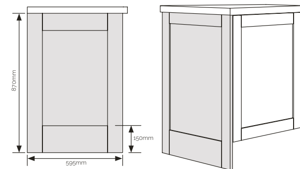
Island framed end panels 595mm - 900mm
