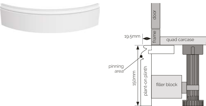
Quadrant pure curve plinth application Ref: PREFIX-CURMPLINTHSCD
