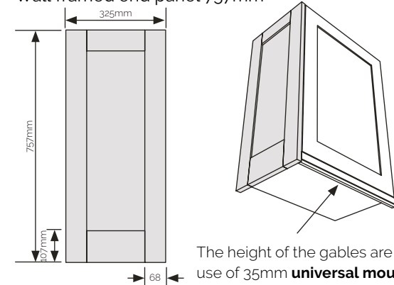
Wall framed end panel 757mm
