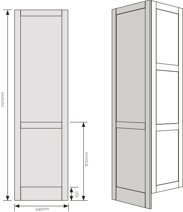
Larder framed end panel 2120mm
