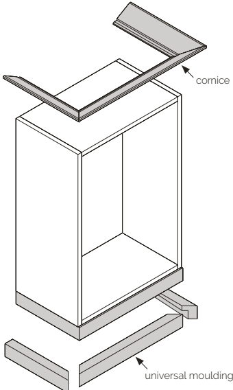
Cornice and pelmet application
