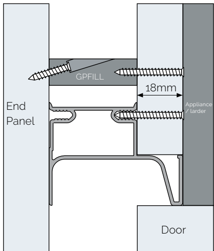
Using Pocket Screws
