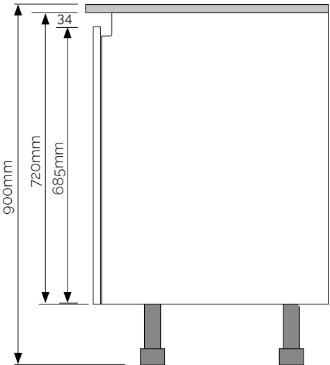
Cabinet dimensions
