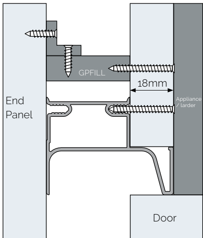
Using an Angle Bracket
